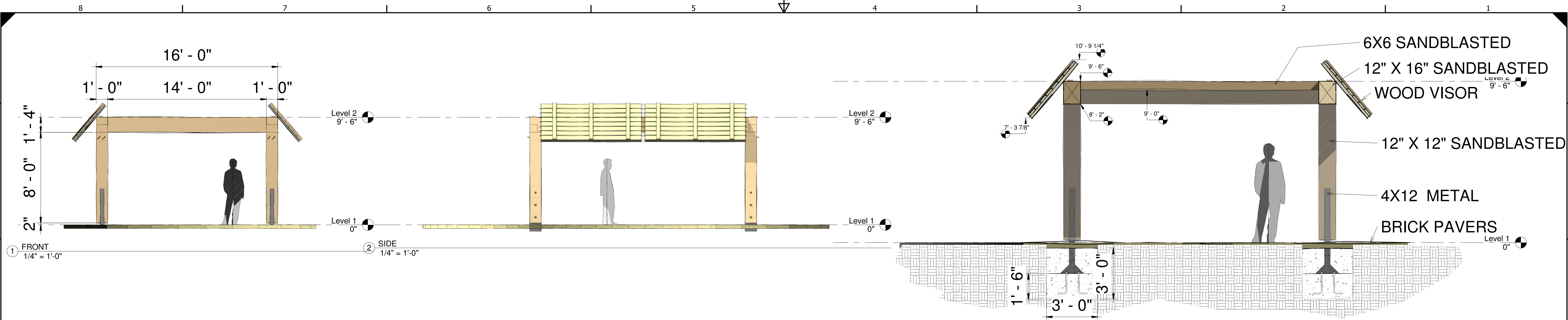
④ Section 1 3/8" = 1'-0"
