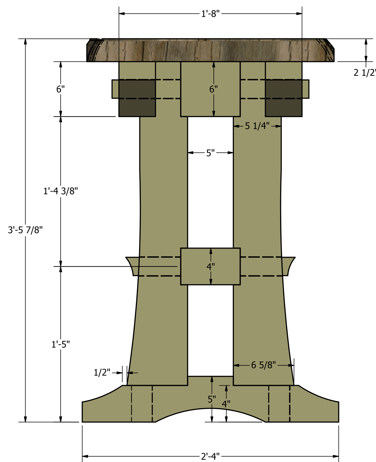
SIDE SCALE 1"=6"
