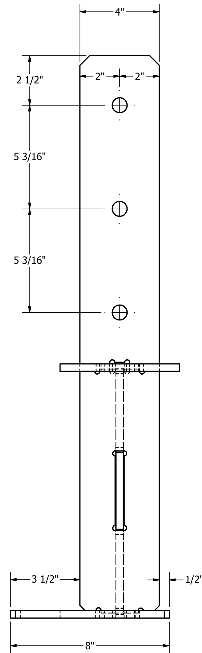
FRONT SCALE 1 / 3
