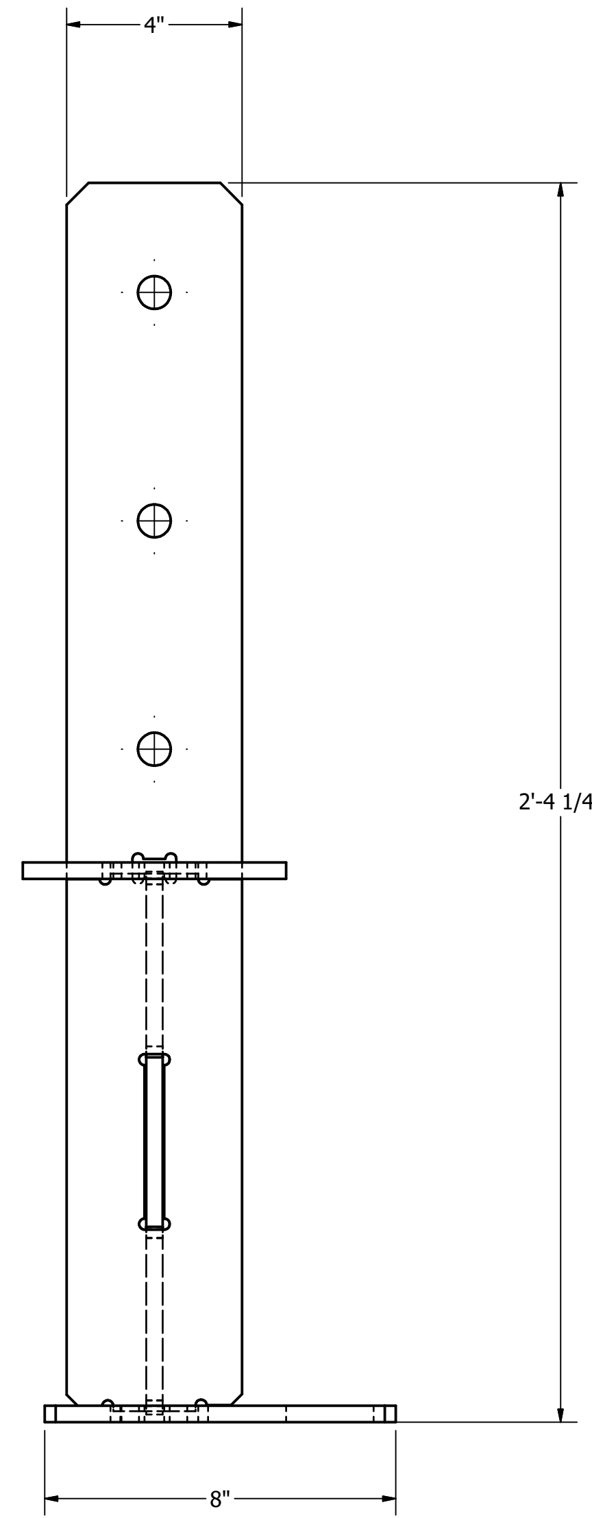
SIDE SCALE 1 / 3
