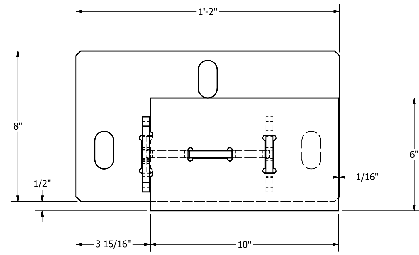
TOP SCALE 1 / 3
