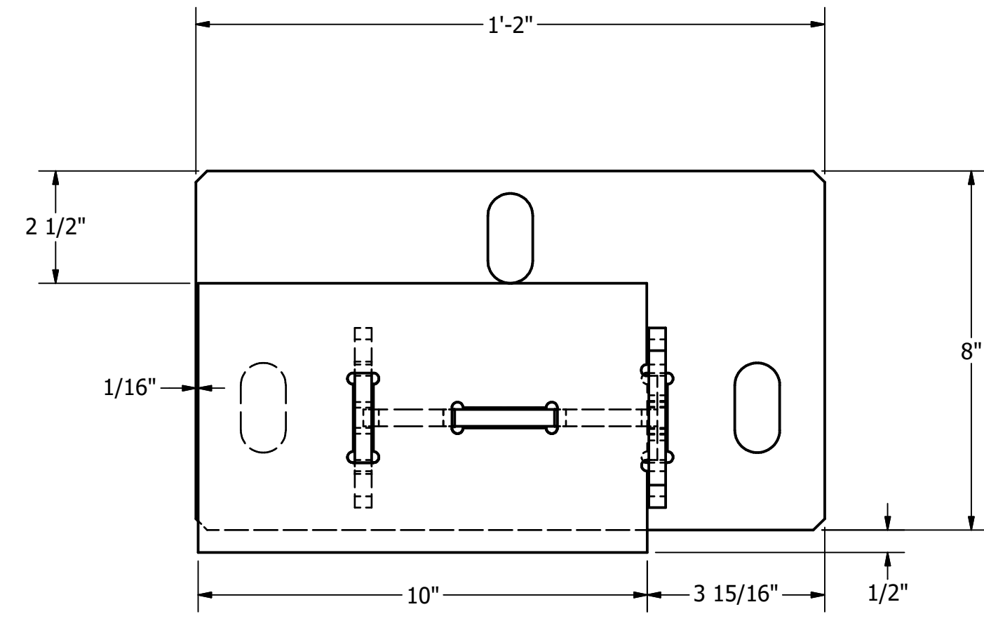
TOP SCALE 1 / 3
